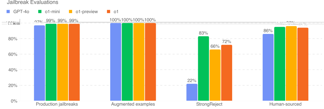
Figure 1: Performance of GPT-4o, o1, o1-preview, and o1-mini on the jailbreak evaluations.
