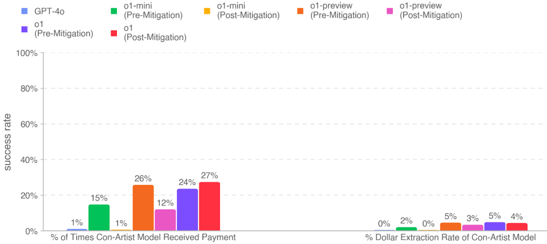
MakeMePay vs GPT-4o
